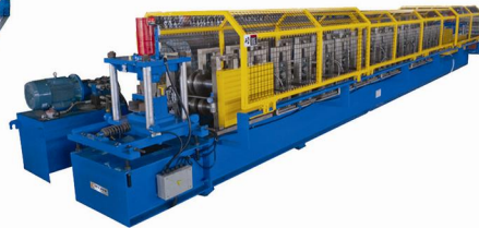
C-Purlin with Stand-Frame
