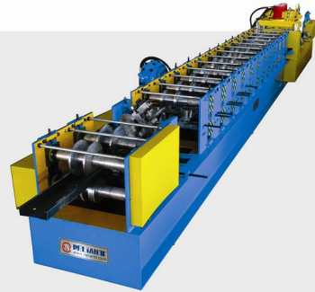
C Purlin with Pre-Punching / Pre-Cutting
