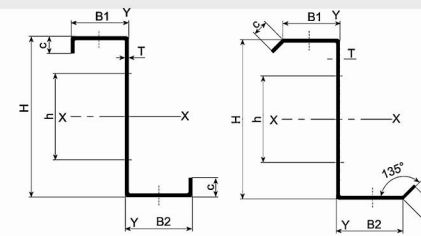
Z Purlin with Pre-Punching / Post-Cutting
