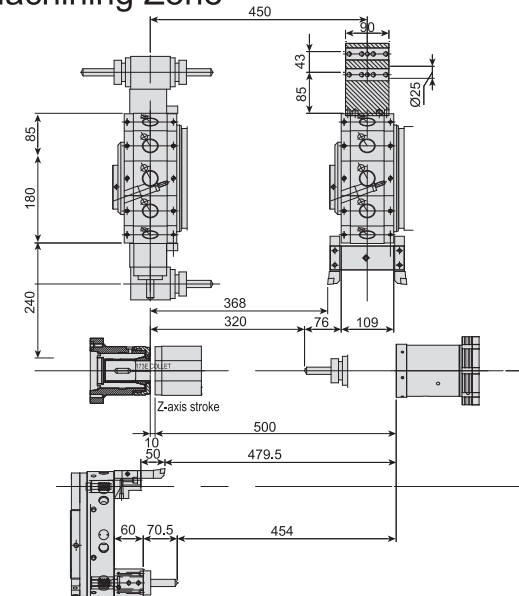
Machining Zone
