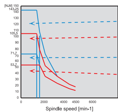
DT FANUC Spindle Motor Torque
