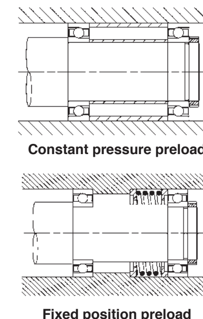
Fig. 5.1 Preloading methods for bearings
