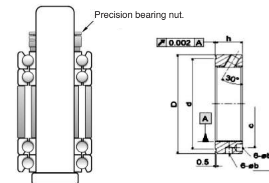
Fig. 8.3 Tightening with precision bearing nut
