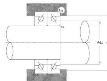
Back-to-back (DB)
