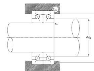
Face-to-face (DF)
