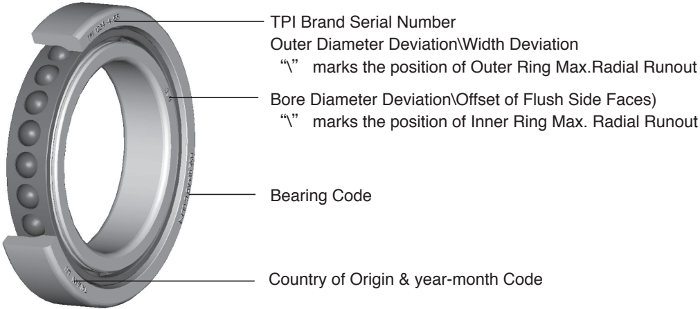
Fig.2.1 Bearing marking designation
