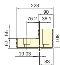
Hardened jaw HJ-40-79
