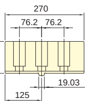
Soft jaw SJ-40-79
