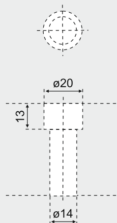
M12 Cap-Screw hole
